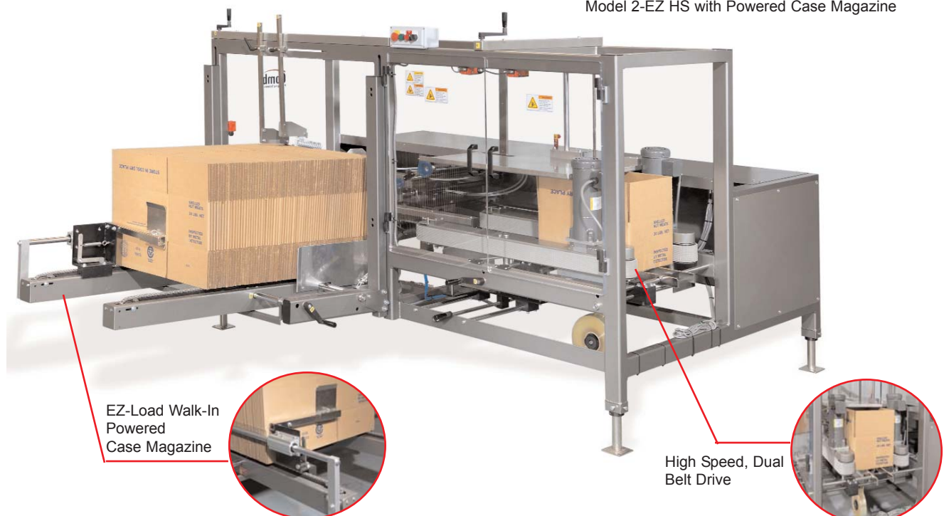
Model 2-EZ HS with Powered Case Magazine
