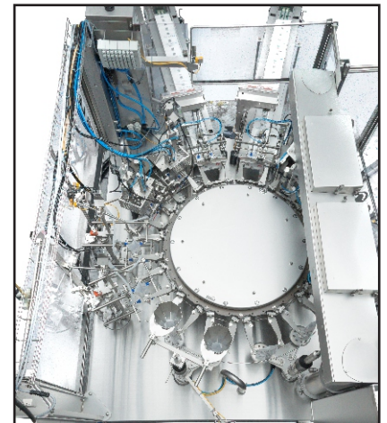
PSG LEE Duplex Pouch Fill-seal Machine
