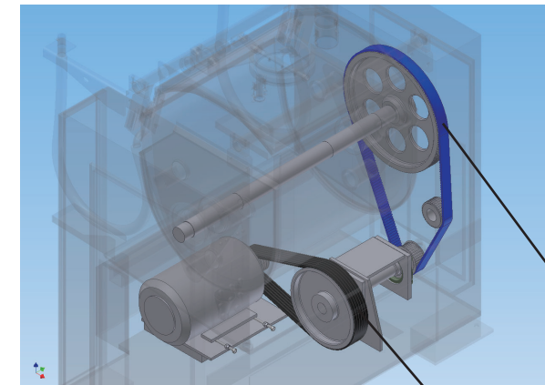
Drive Mechanism
