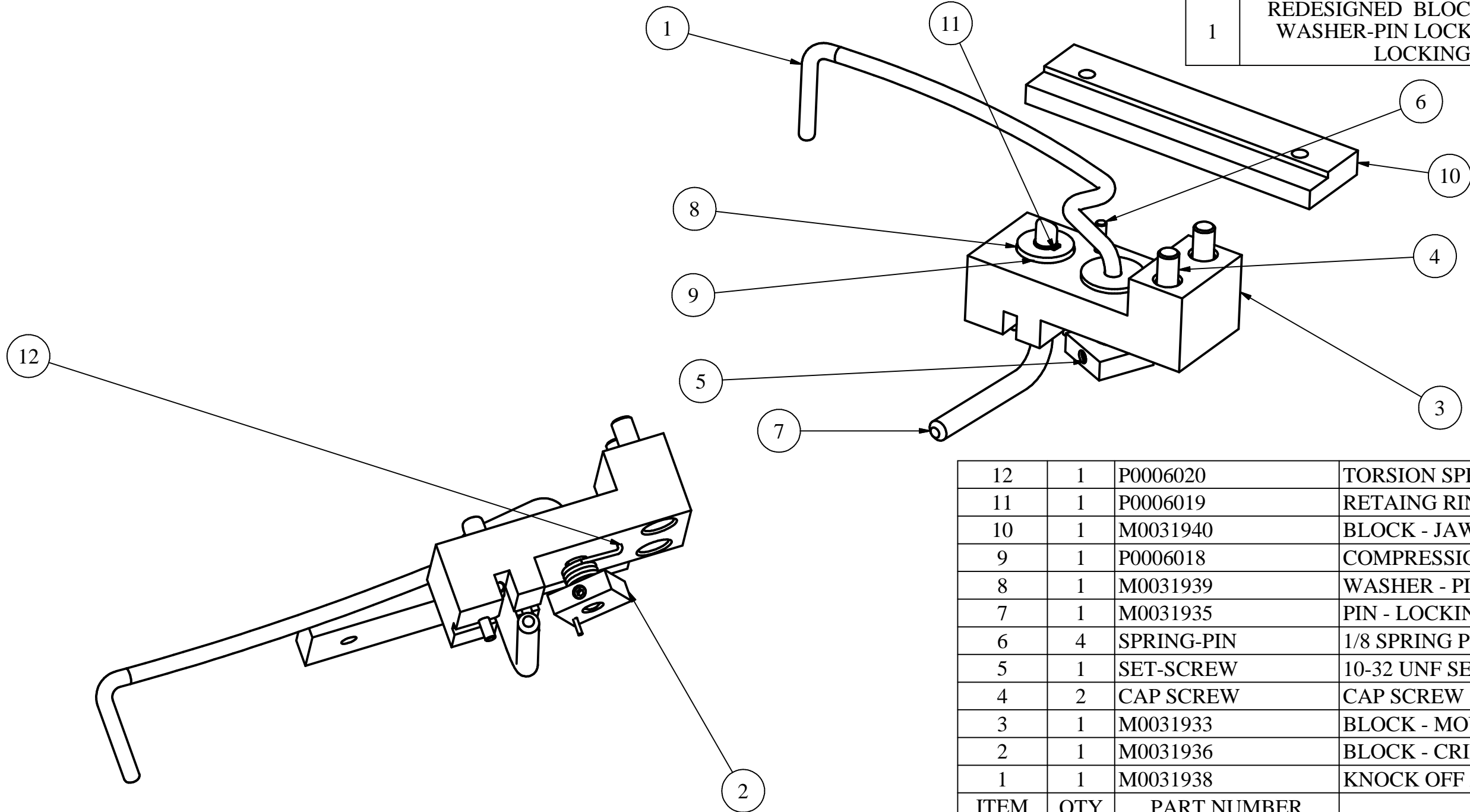
Parts List
